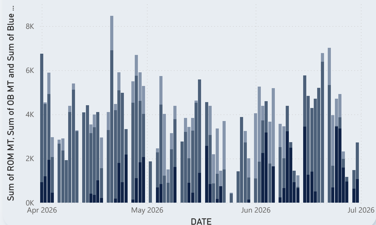
Material Composition by Day
