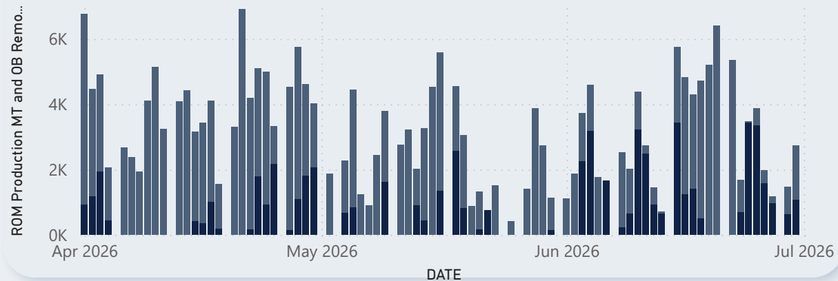
Daily ROM Mined vs. OB Removed (MT)
