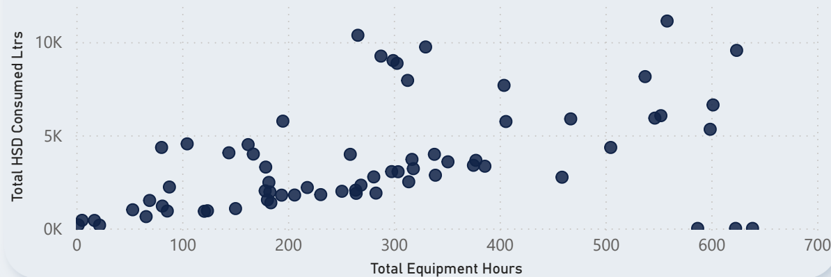
HSD Consumed vs. Running Hours by Machine
