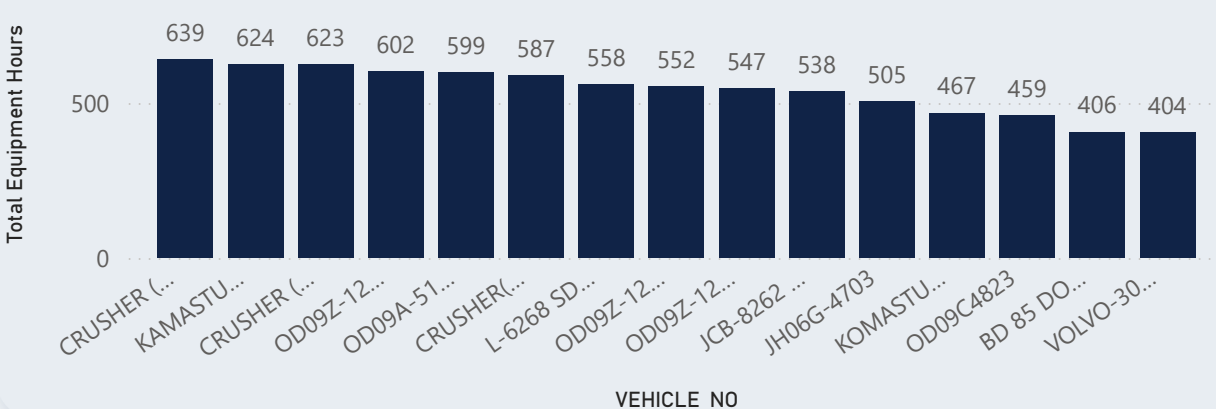
Running Hours by Equipment
