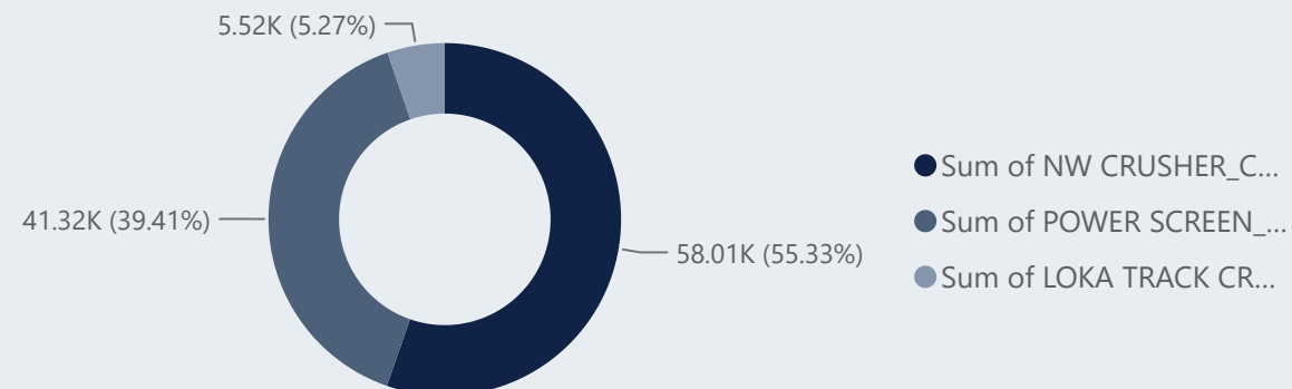
Production by Crusher Plant
